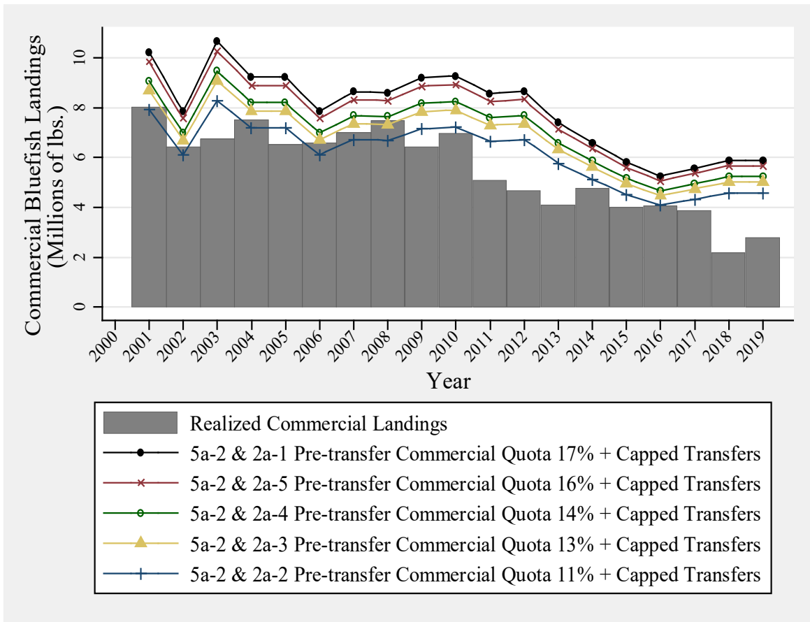
Figure 26: Realized commercial bluefish landings and predicted commercial landings under the 10% ABC cap transfer scenario across proposed commercial allocation alternatives from 2001-2019.
