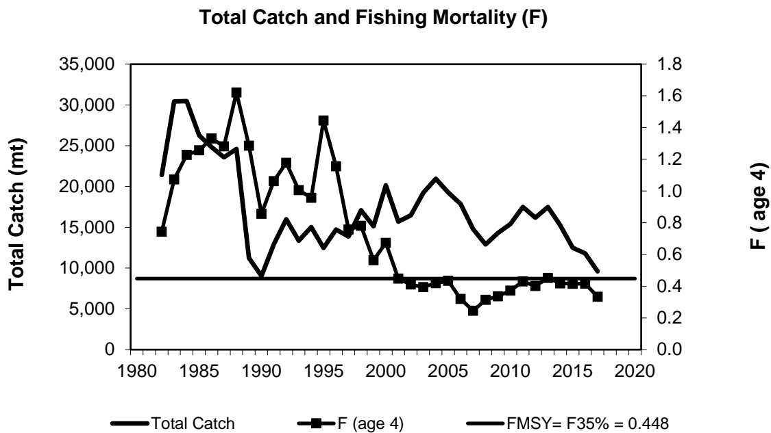
Figure 4: Total fishery catch (mt) and fully-recruited fishing mortality (peak at age 4) of summer flounder. The horizontal solid line is the fishing mortality reference point proxy FMSY = F35% = 0.448 (NEFSC 2019).
