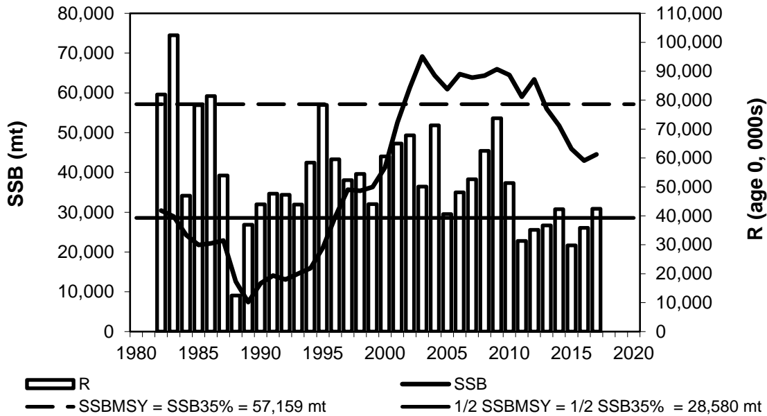
Figure 5: Summer flounder SSB and recruitment at age 0, 1980-2017. The horizontal dashed line is the target biomass reference point proxy, SSB_{MSY} = SSB_{35\%} = 57,159 mt. The horizontal solid line is the threshold biomass reference point proxy \frac{1}{2} SSB_{MSY} = \frac{1}{2} SSB_{35\%} = 28,580 mt (NEFSC 2019).
