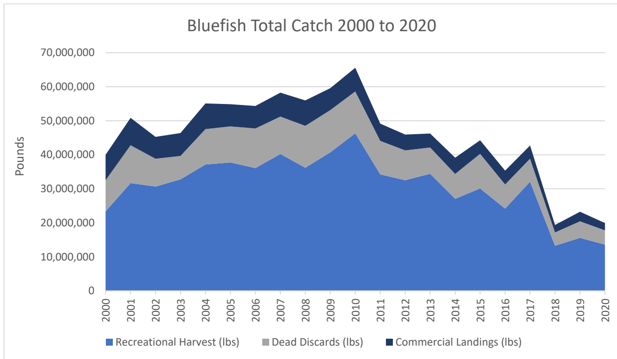
Figure 2. Bluefish catch (landings [AB1] and dead discards [B2*0.15*Avg wt. each year]), 2000-2020. Recreational dead discards are calculated as the average weight of a harvested fish by year, state and mode multiplied by the B2s and 15% discard mortality rate (Source: MRIP and Dealer data – cfders)
