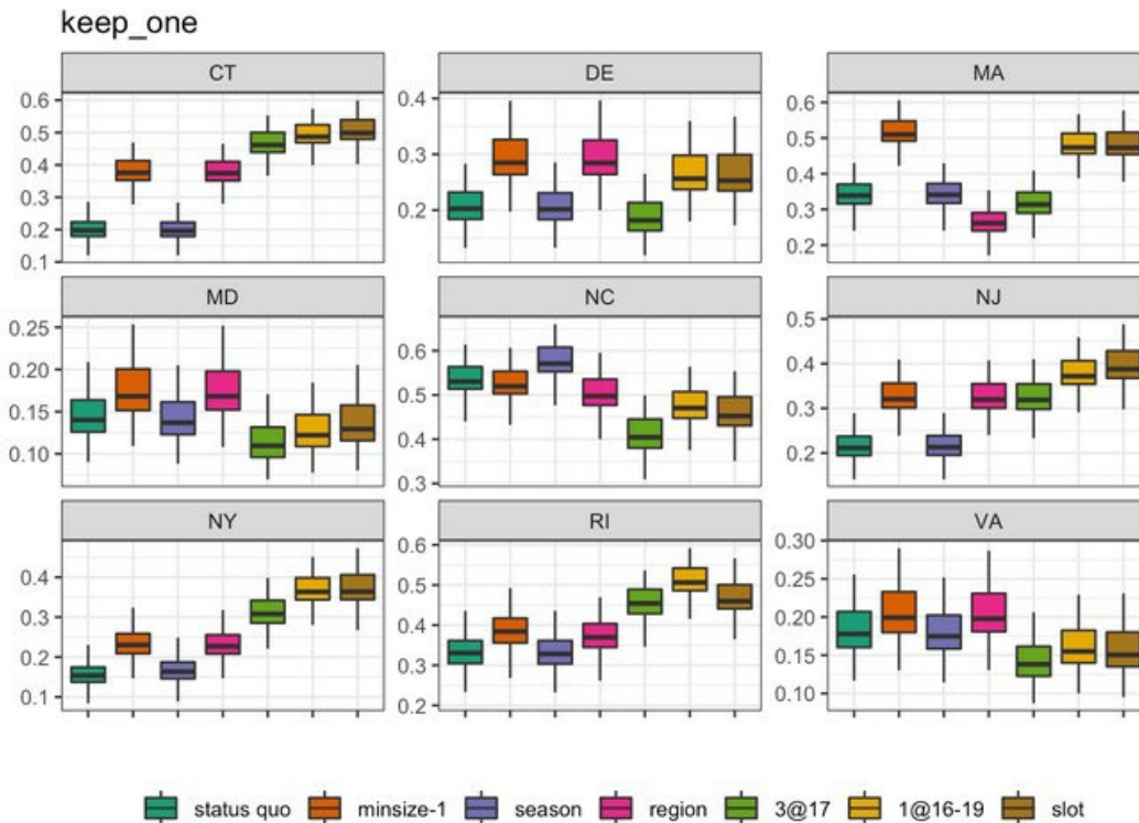
Figure 3. Comparison of the average number of trips where one summer flounder was kept across the seven different management procedures for each state under the baseline operating model.
