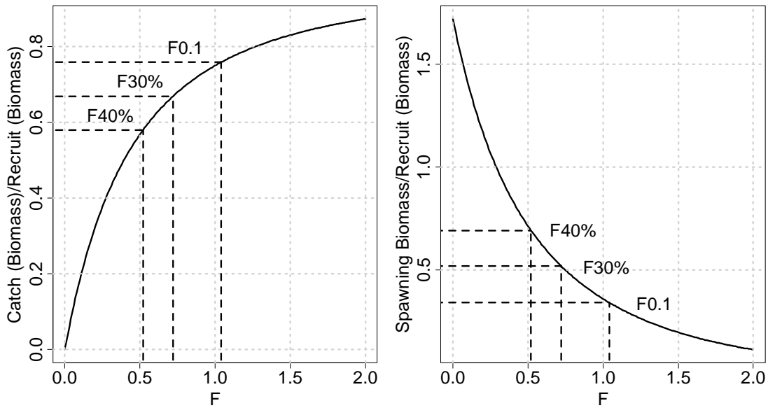
Figure B4. Equilibrium ratio of catch and spawning biomass to recruit biomass given constant fishing mortality on butterfish.
